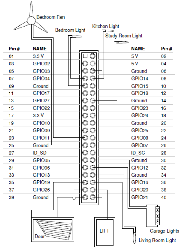
Figure 5. Circuit of the whole hiko system [3]
