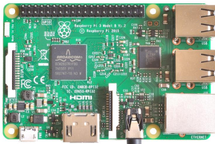
Figure 1. Raspberry Pi 3 Model B[7]
